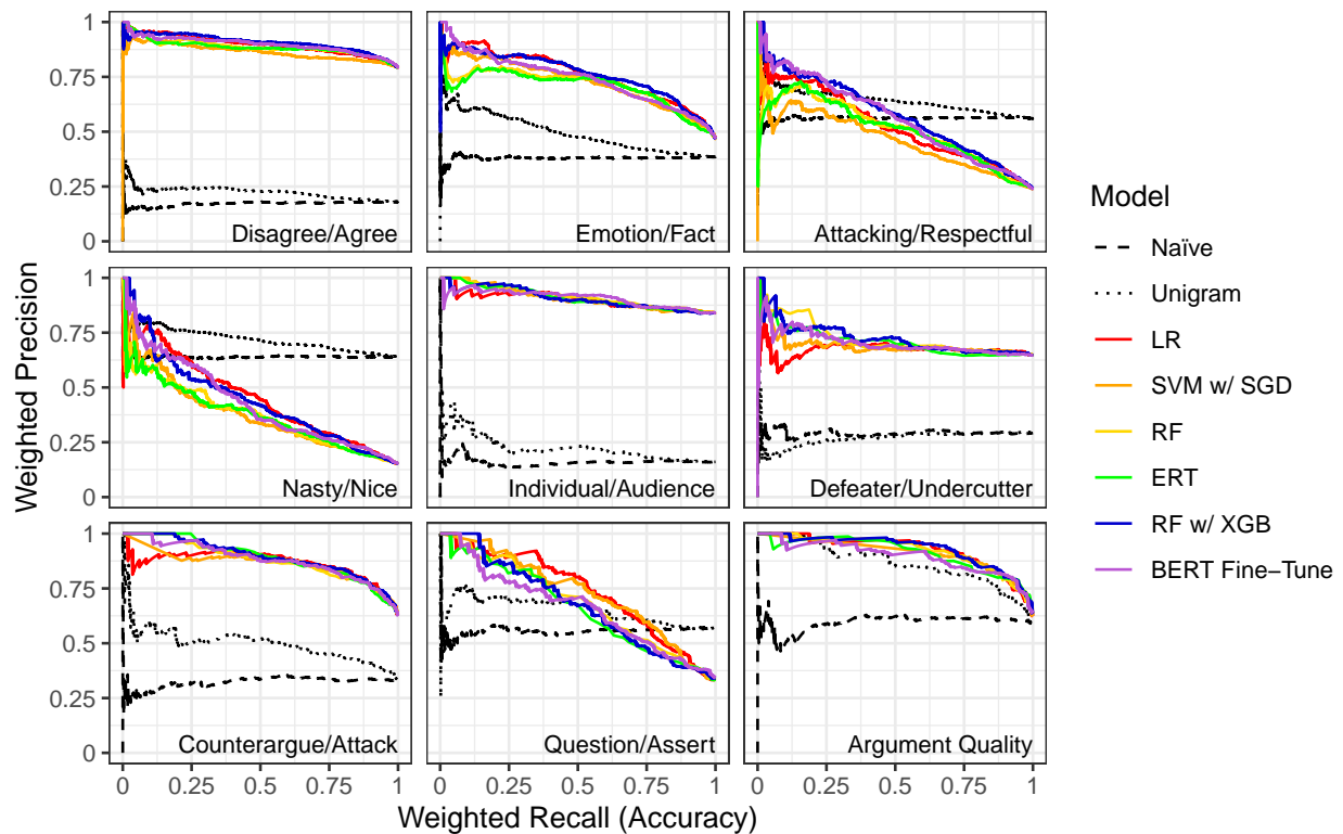
Figure S1: Weighted Precision and Recall Curves. Weighted recall is mathematically equivalent to accuracy. Black curves represent baselines, colored curves represent deep learning models.
