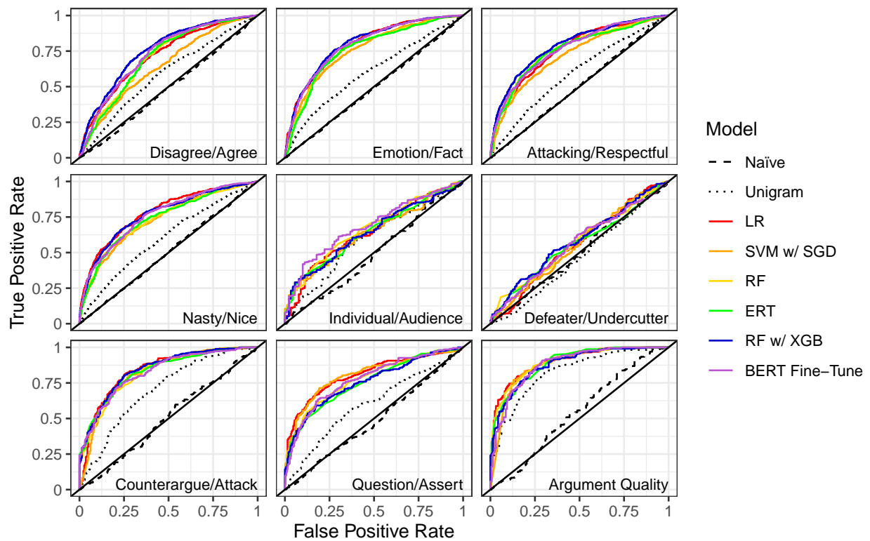
Figure S2: Receiver-Operating Characteristic Curves. Black curves represent baselines, colored curves represent deep learning models.
